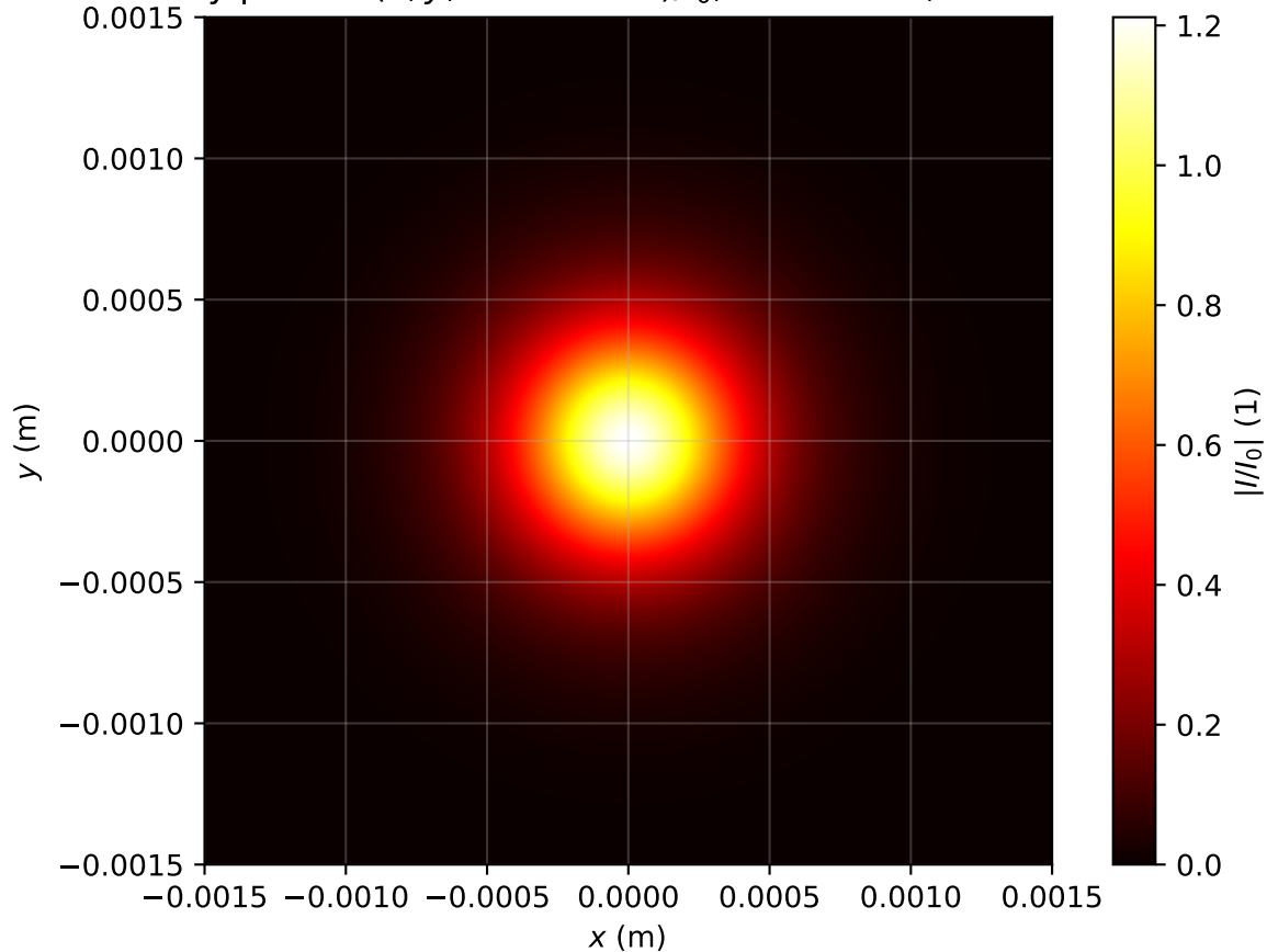
Intensity profile I(x, y, z = 1.194m)/I_0 , P_{in}=0.7P_{cr} , artificial time
